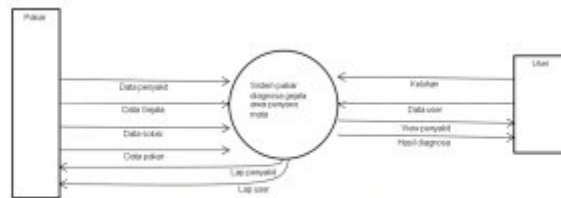
Gambar 4.4. Context Diagram
