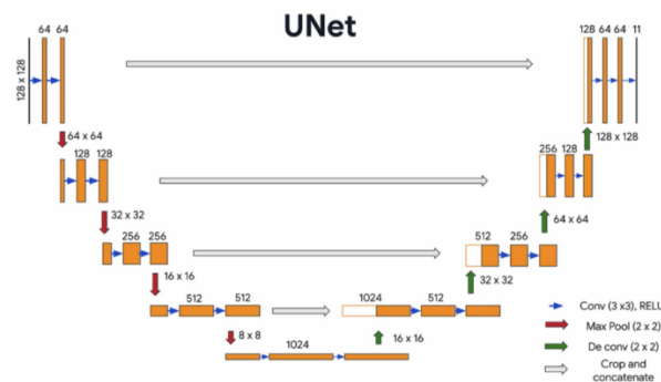
Figure 1. U-Net Architecture
