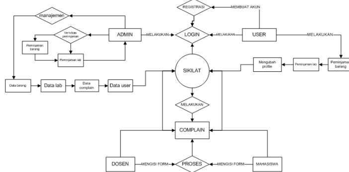
Gambar 1. Gambar Erd database
